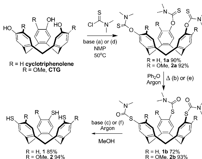
Scheme 2. The synthesis of cyclotrithiophenolene 1 and cyclotrithioguaicylene 2 . Additional details of conditions for 1 : a) Cs 2 CO 3 ; b) 305 °C; c) 4 M KOH. Additional details of conditions for 2 : d) DABCO; e) 255 °C; f) 4 M NaOH. DABCO = 1,4-diazabicyclo-[2.2.2]octane.
